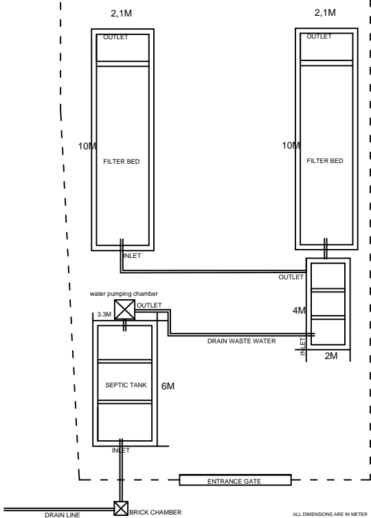
PLAN LAYOUT
