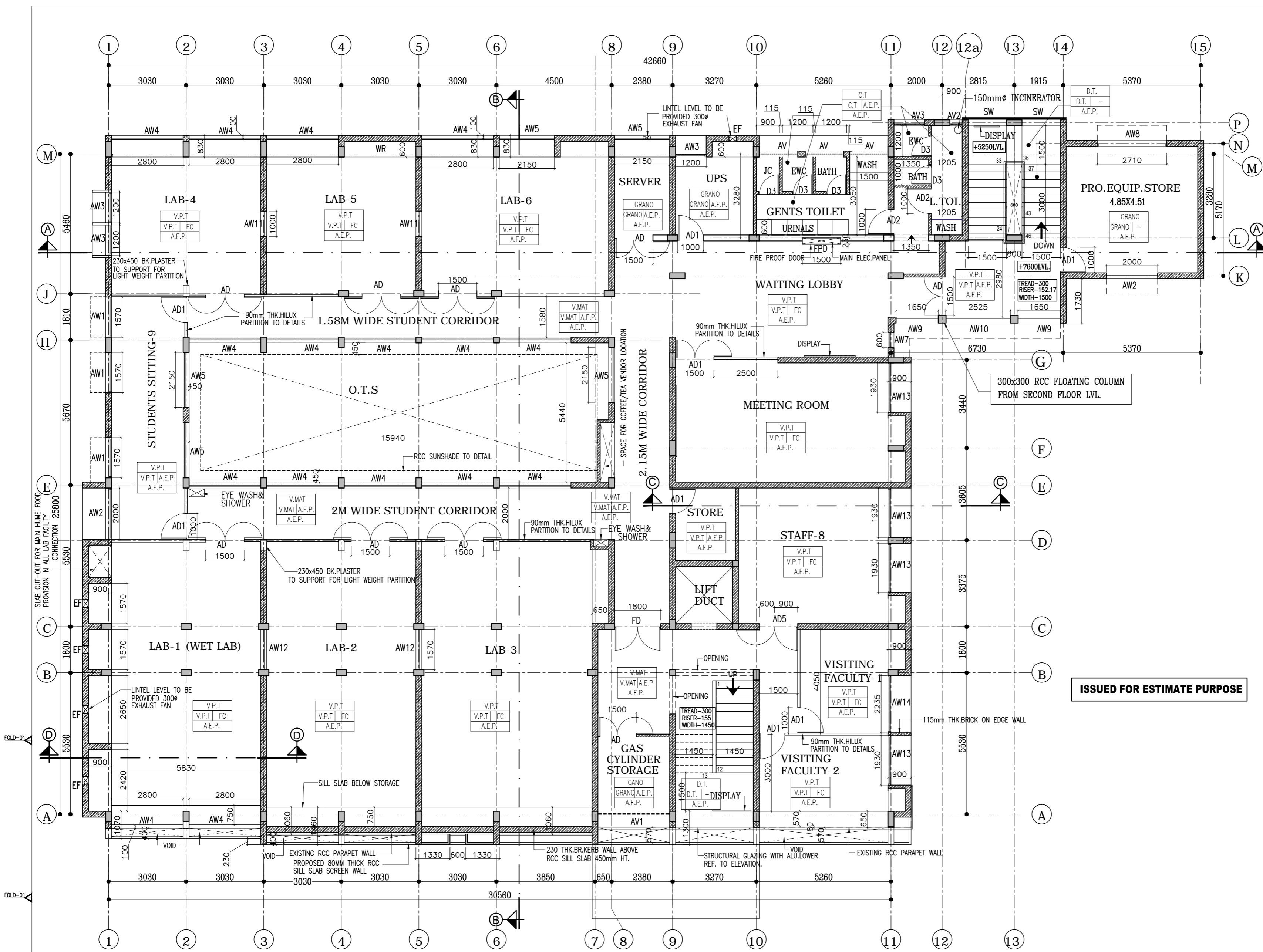
PRO. SECOND FLOOR PLINTH AREA - 855.00 SQM (OR) 9200 SQFT.
