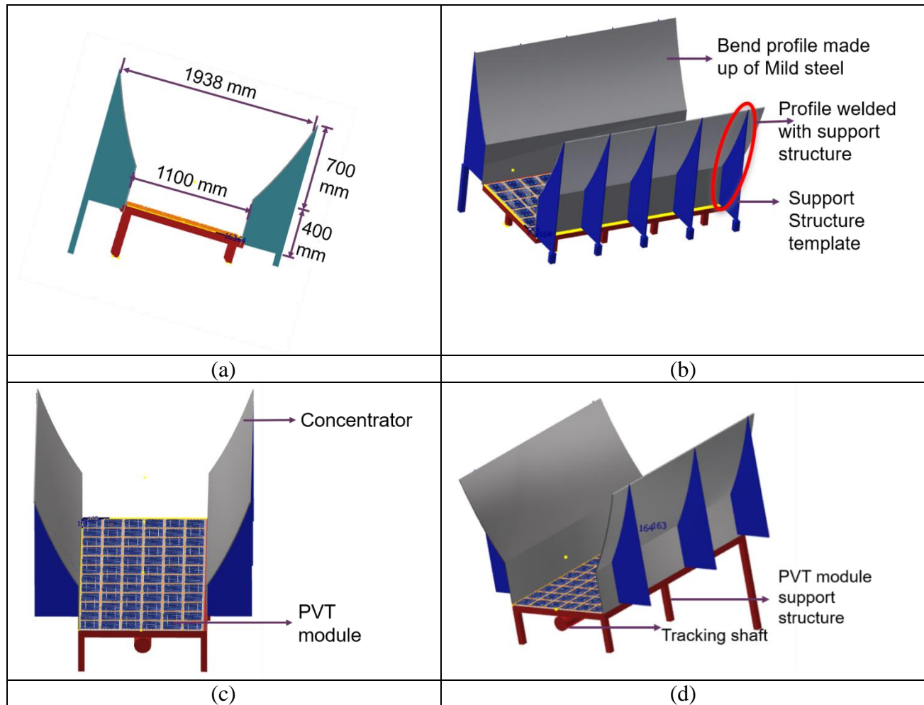
LCPVT system configuration.
