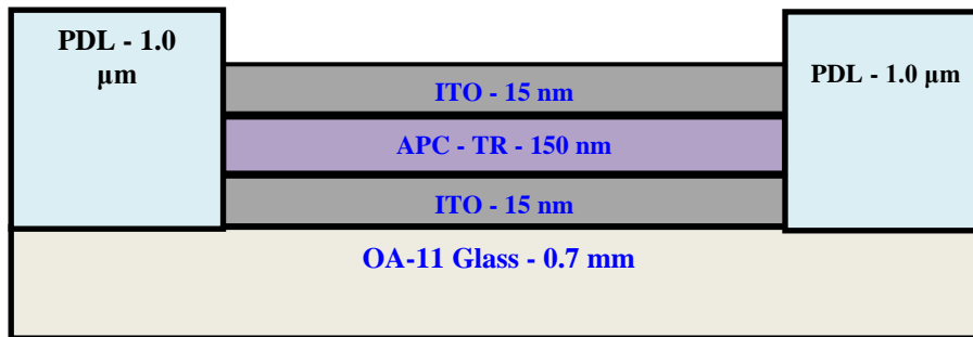
Figure 2: Substrate cross section view
