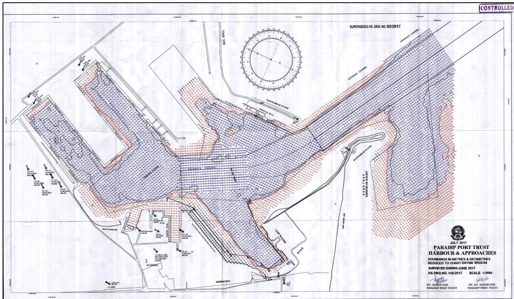
Fig No 1. Paradip Port Bathymetry Chart
