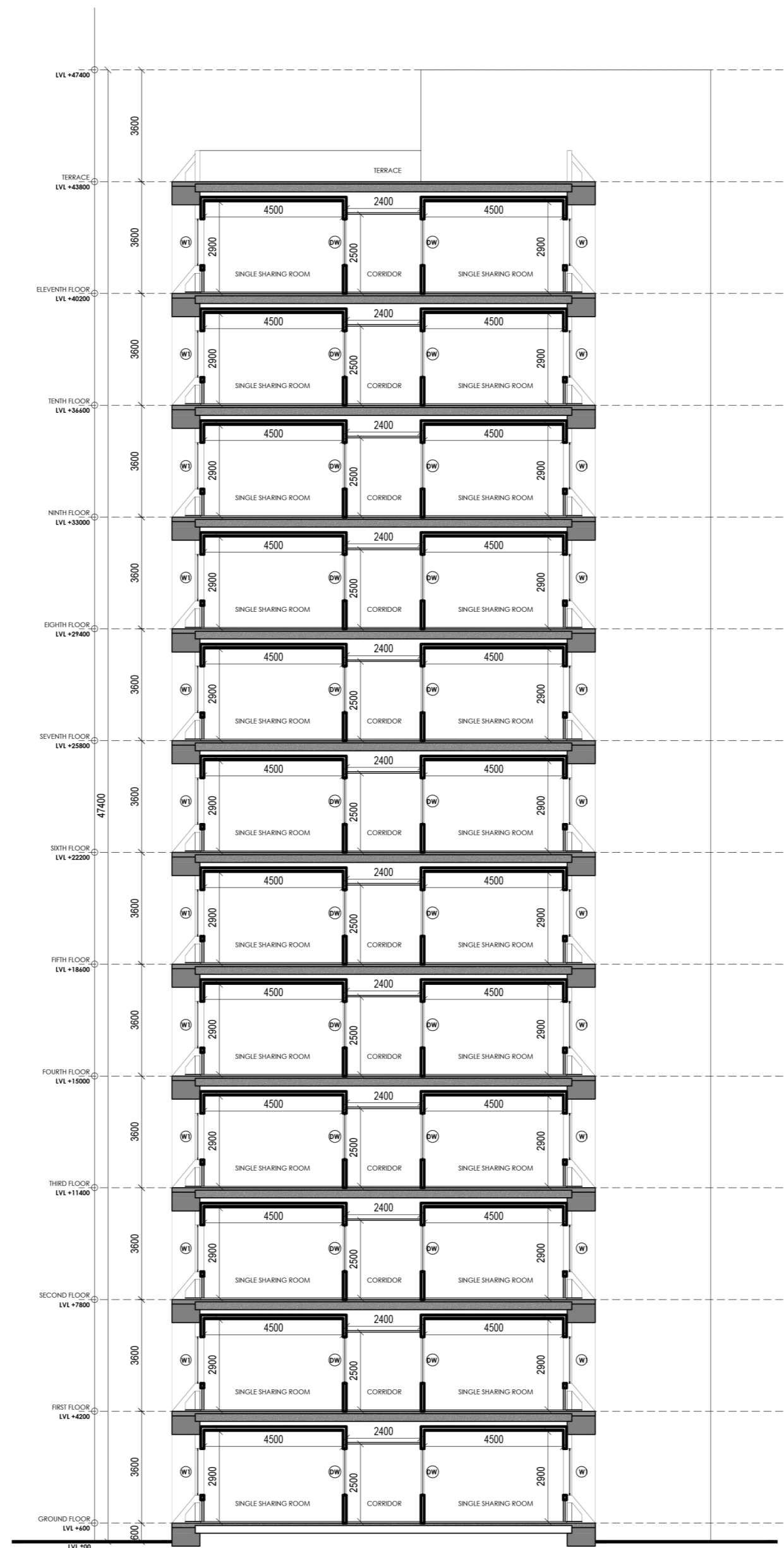
DETAILS OF SECTION A-A OPTION-1
