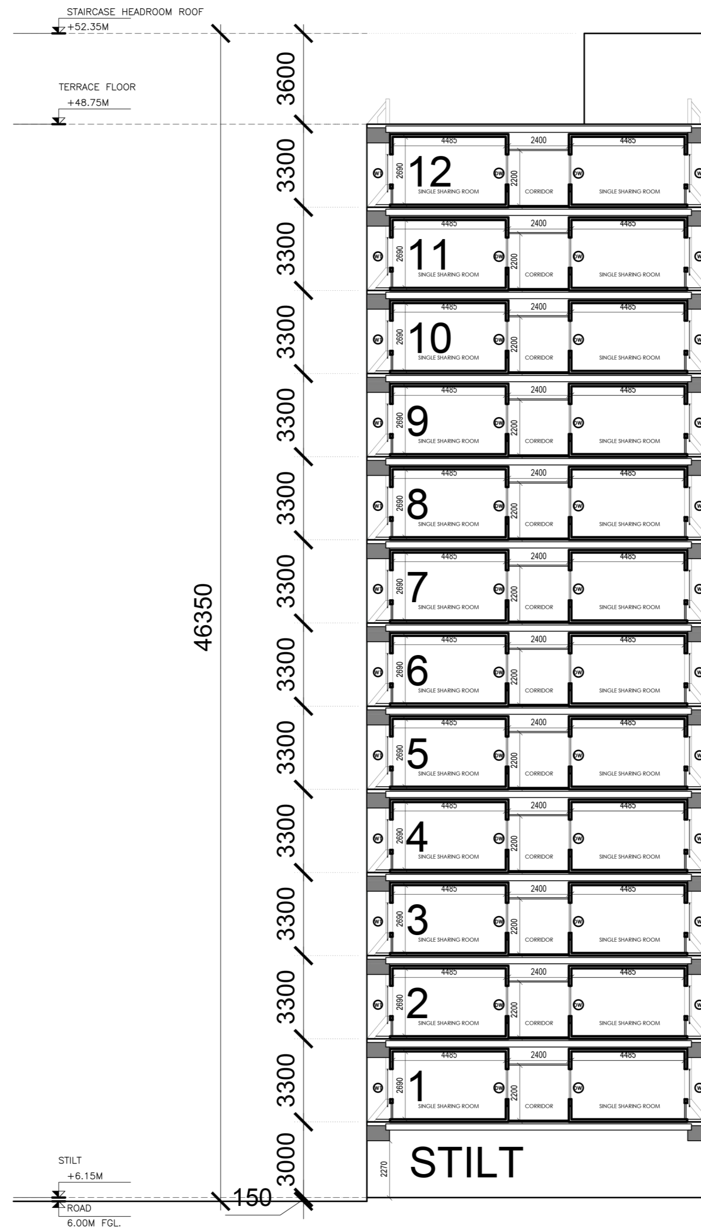
DETAILS OF SECTION A-A OPTION-2
