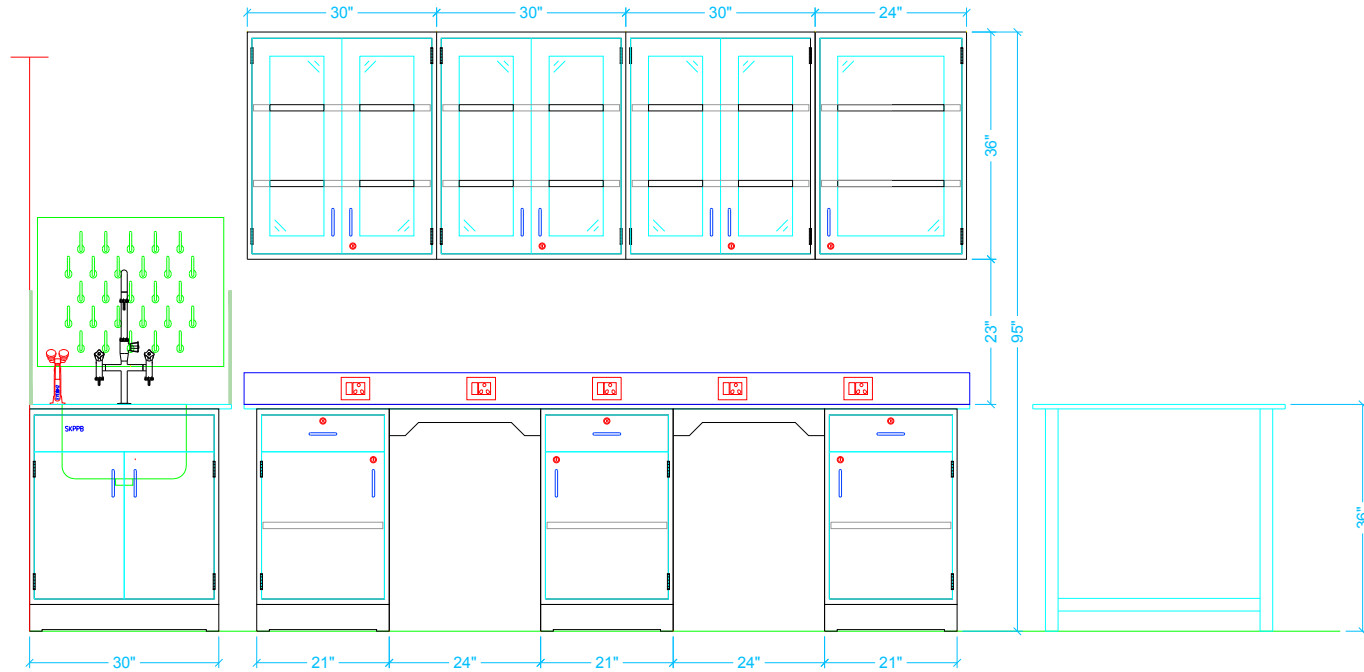
Elevation-1
