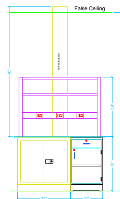
Elevation-3
