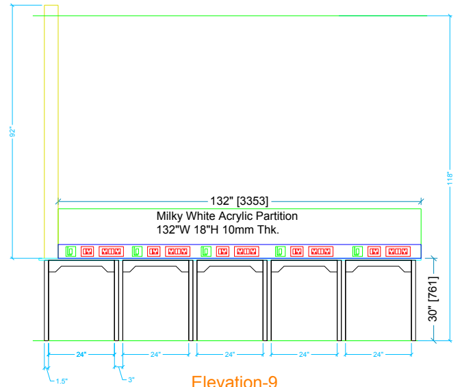
Elevation-9
