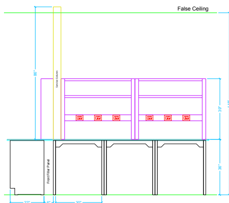
Elevation-2
