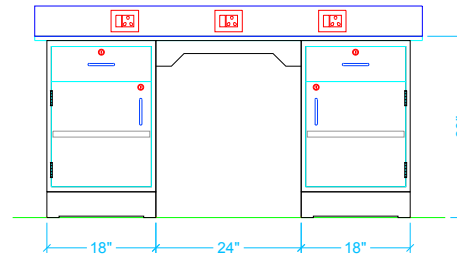
Elevation-5
