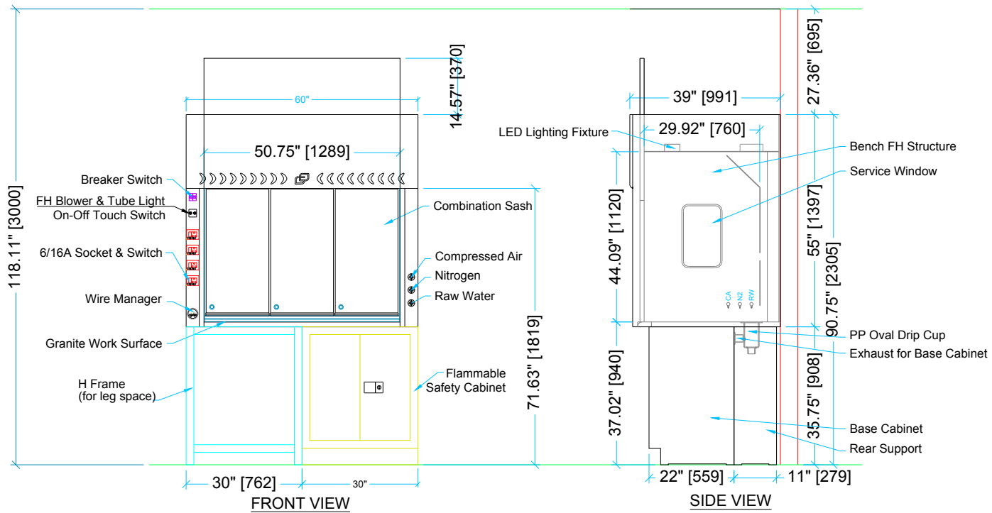
BENCH FUME HOOD 60"W x 40"D x 90.75"H
