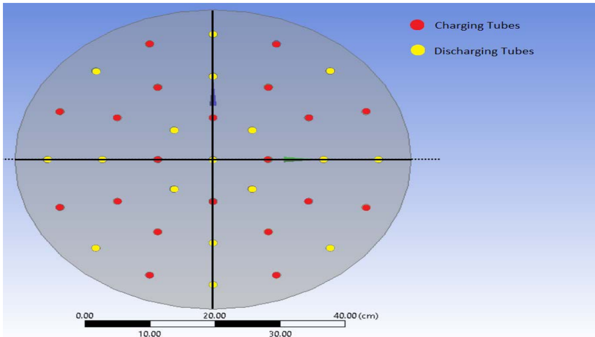
Fig. 6 Tube arrangement for fourth stage TES system.
