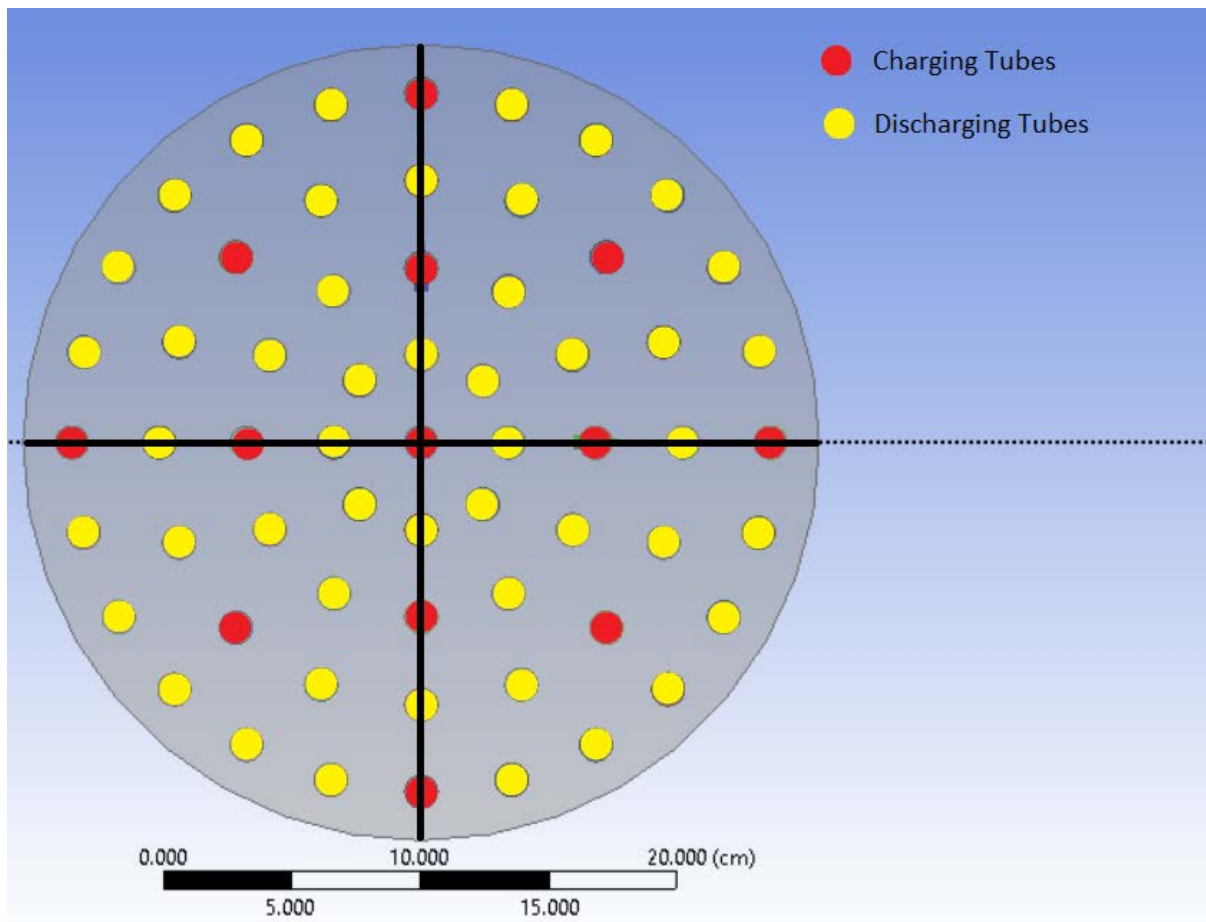
Fig. 5 Tube arrangement for third stage TES system.
