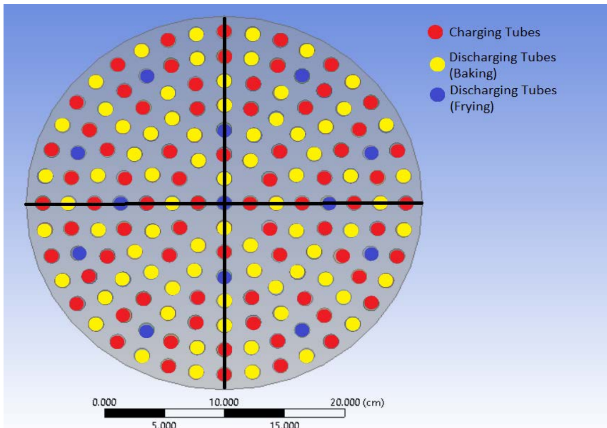
Fig.2 Tube arrangement for first stage TES system.
