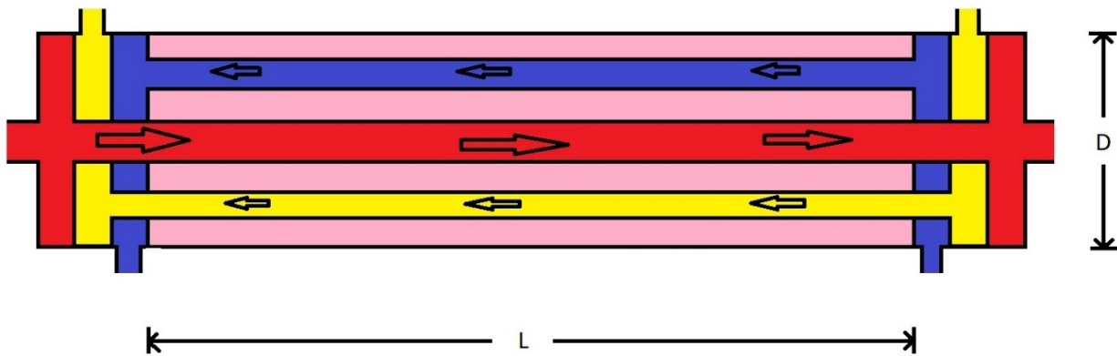
Fig. 1 Layout for only first stage thermal energy storage system.
