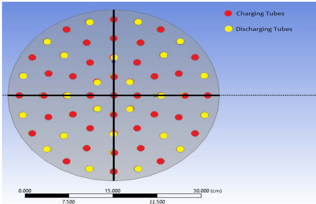
Fig. 4 Tube arrangement for second stage TES system.
