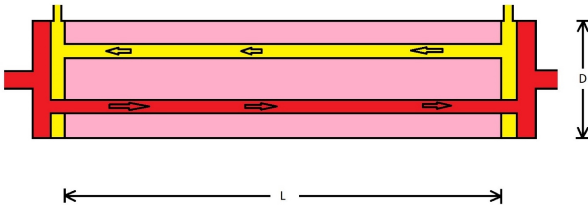
Fig.3 Layout for other three stage thermal energy storage system.
