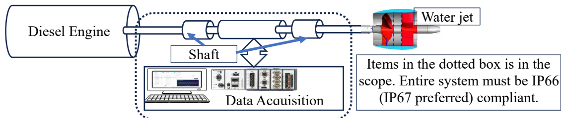
Fig. 1 Block schematic of Torque-Thrust-RPM Sensor System
