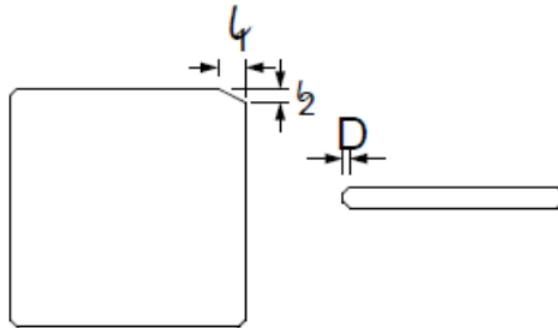
Figure 1: The film side of the substrate shows that the orientation corner(1C) is located at the top righthand side.
