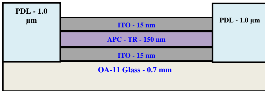
Substrate section view
