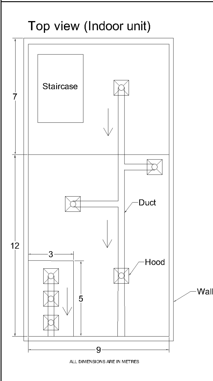
Fig 1: Top view of the exhaust system components inside the laboratory
