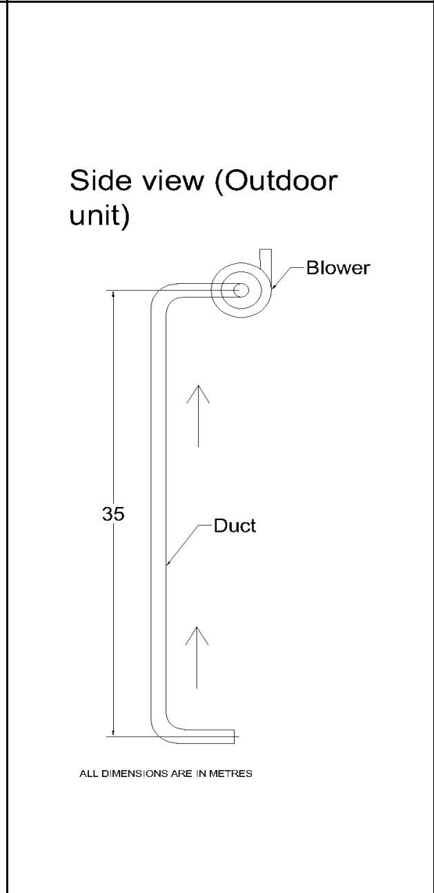
Fig 2: Side view of the exhaust duct connected to the blower outside the laboratory
